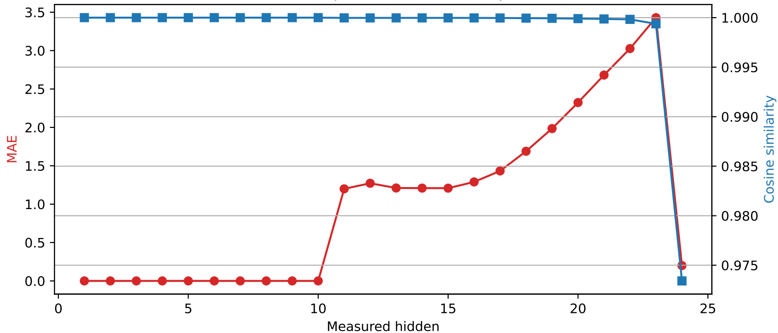
SmolLM2-1.7B-Instruct | Quantized layer 10 | float64 → int2
