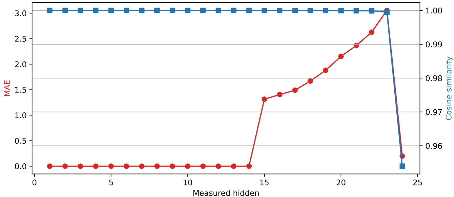
SmolLM2-1.7B-Instruct | Quantized layer 14 | float64 \rightarrow int2
