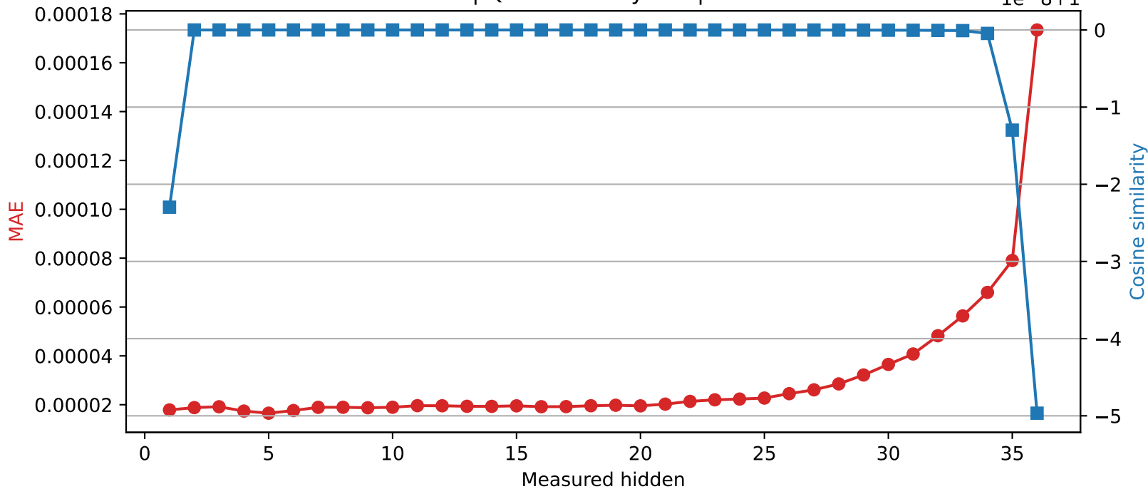
SmolLM3-3B | Quantized layer 0 | float32 → int16
