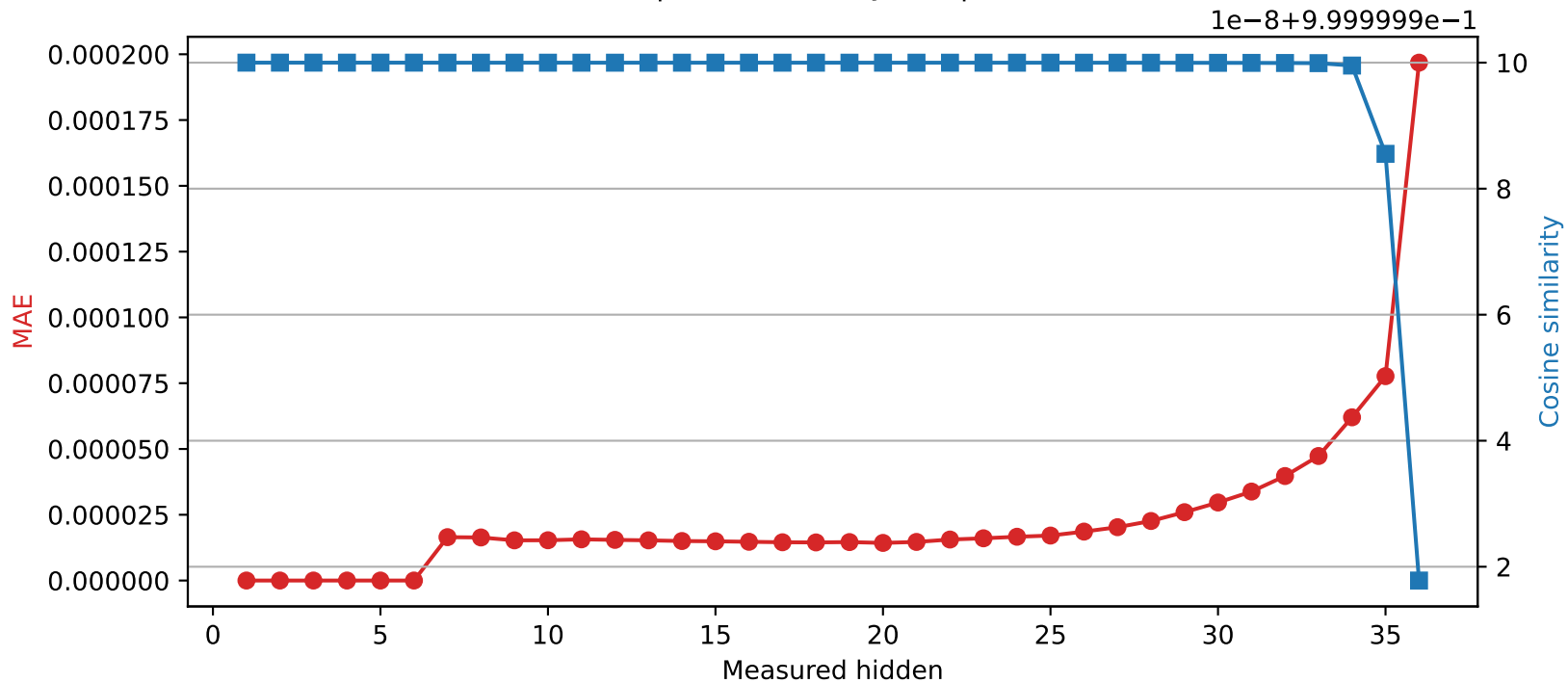
SmolLM3-3B | Quantized layer 6 | float32 → int16
