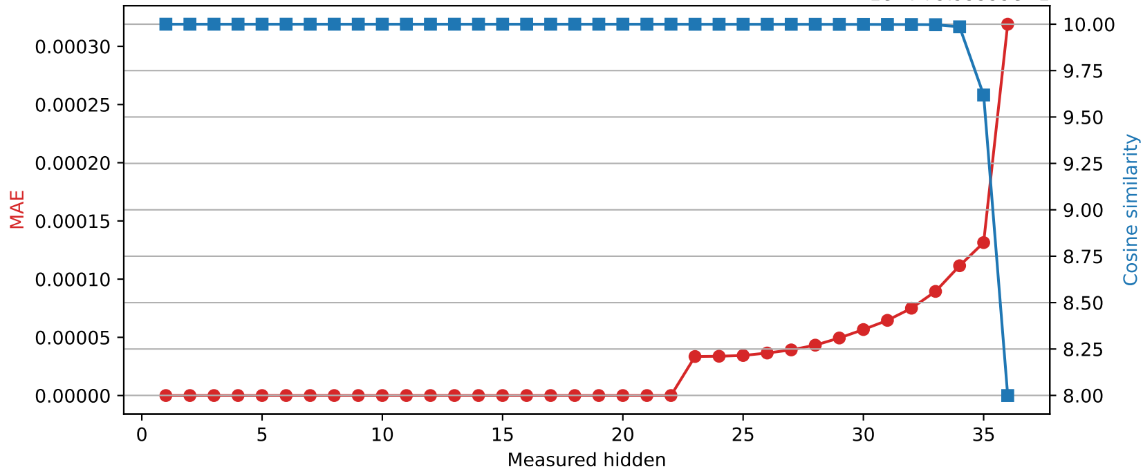
SmolLM3-3B | Quantized layer 22 | float32 \rightarrow int16 1e-7+9.99999e-1
