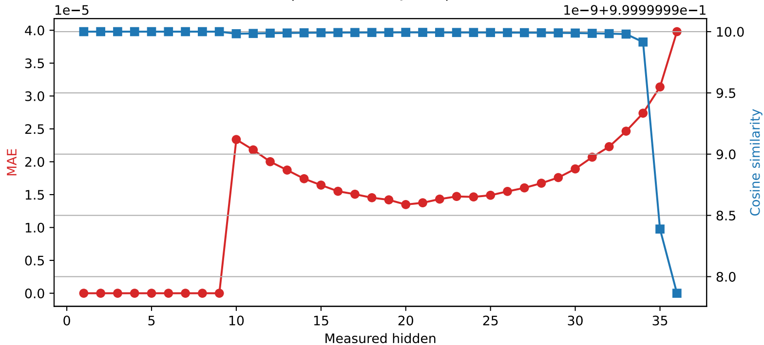
SmolLM3-3B | Quantized layer 9 | float32 → int16
