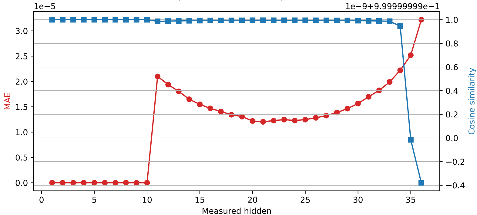
SmolLM3-3B | Quantized layer 10 | float32 → int16
