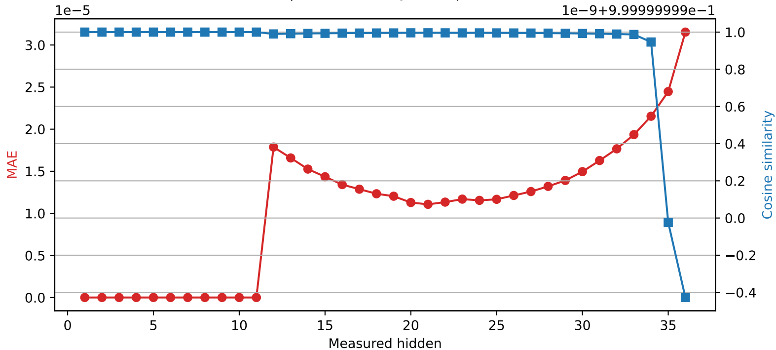
SmolLM3-3B | Quantized layer 11 | float32 → int16
