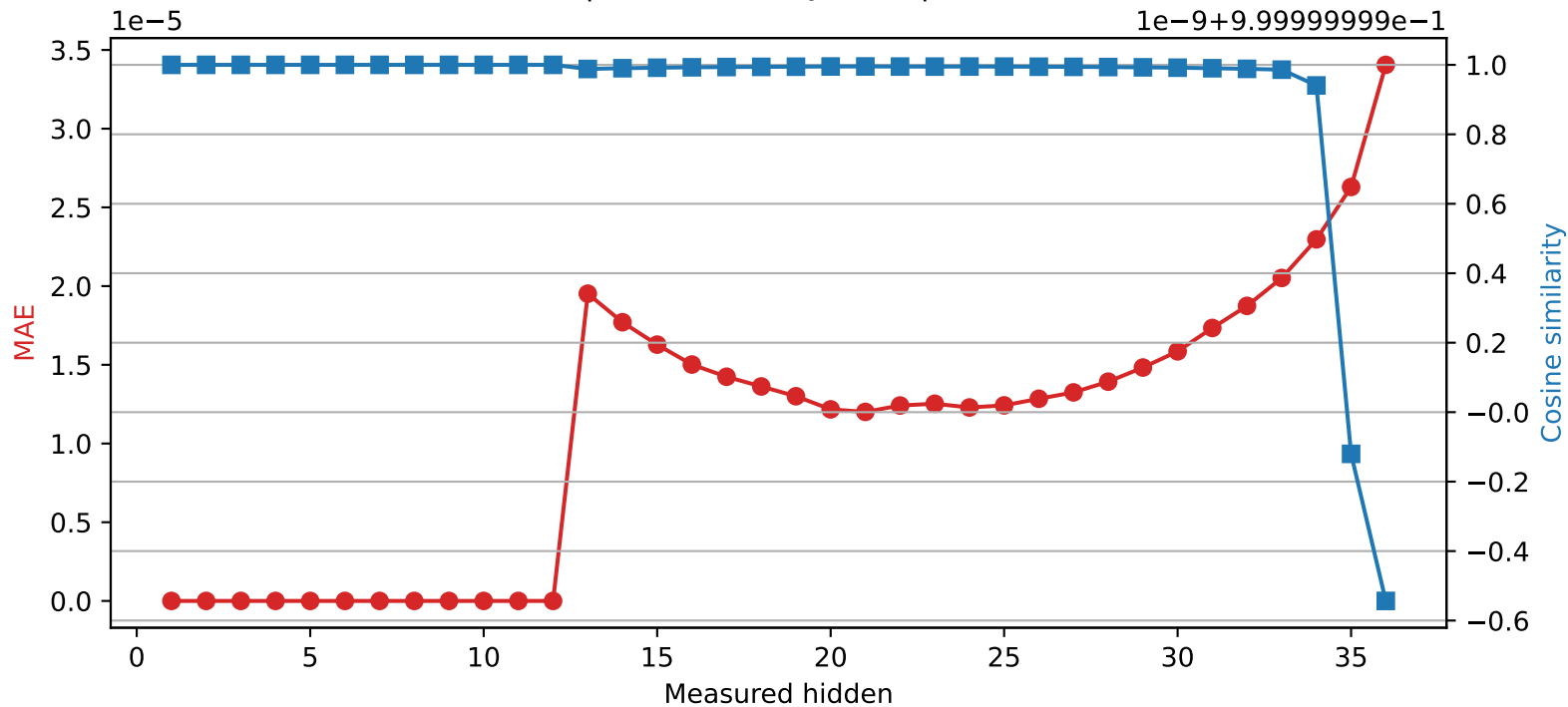
SmolLM3-3B | Quantized layer 12 | float32 → int16
