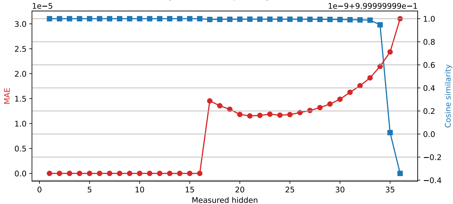
SmolLM3-3B | Quantized layer 16 | float32 → int16
