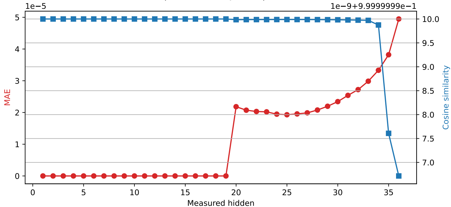
SmolLM3-3B | Quantized layer 19 | float32 → int16
