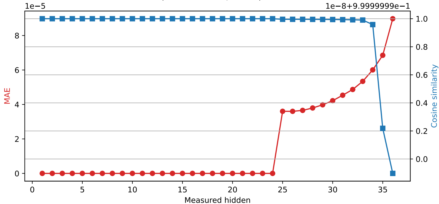
SmolLM3-3B | Quantized layer 24 | float32 → int16
