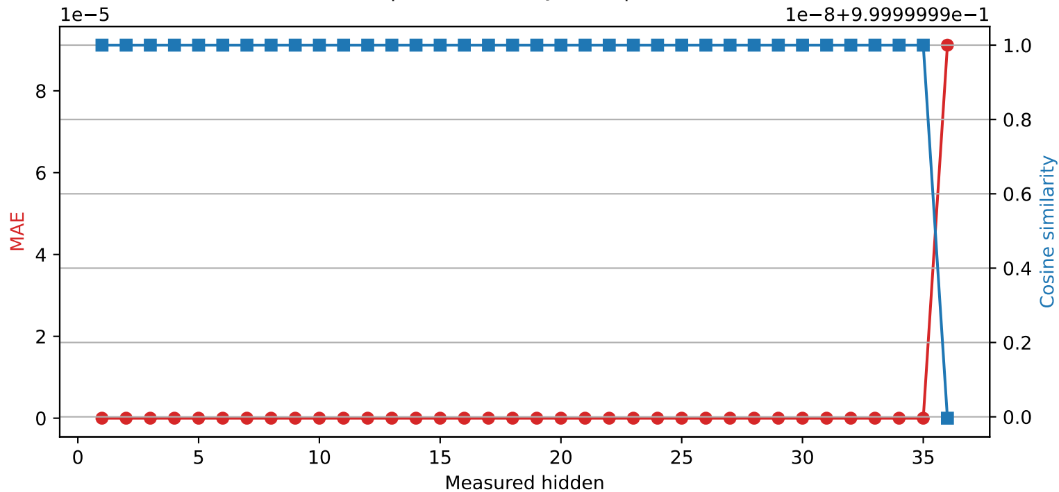
SmolLM3-3B | Quantized layer 35 | float32 → int16
