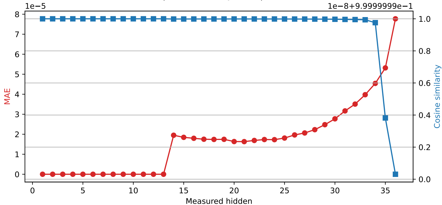
SmolLM3-3B | Quantized layer 13 | float32 → int16
