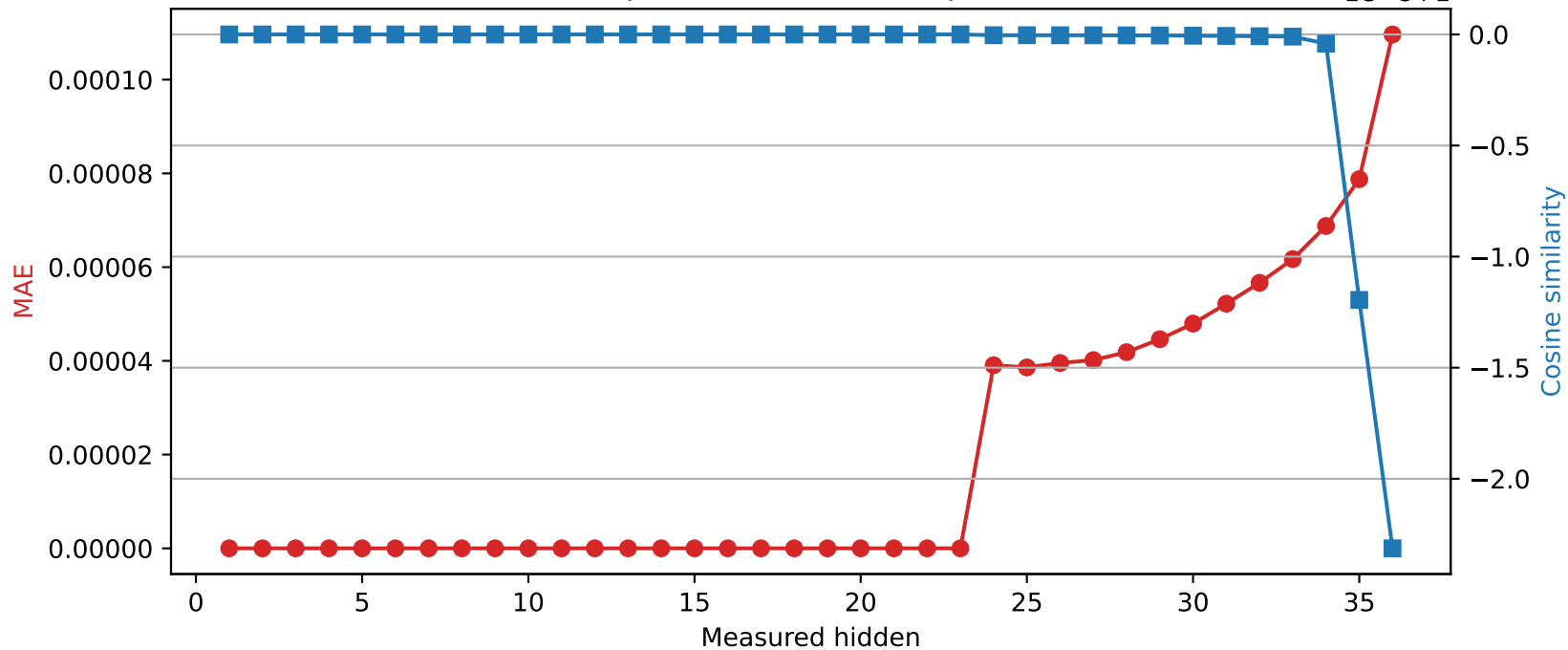
SmolLM3-3B | Quantized layer 23 | float32 → int16
