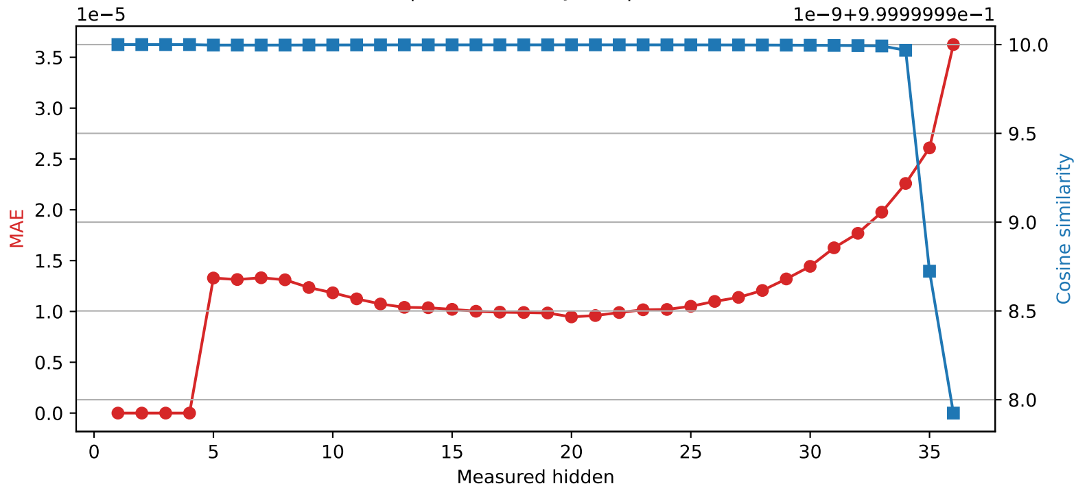
SmolLM3-3B | Quantized layer 4 | float64 → int16
