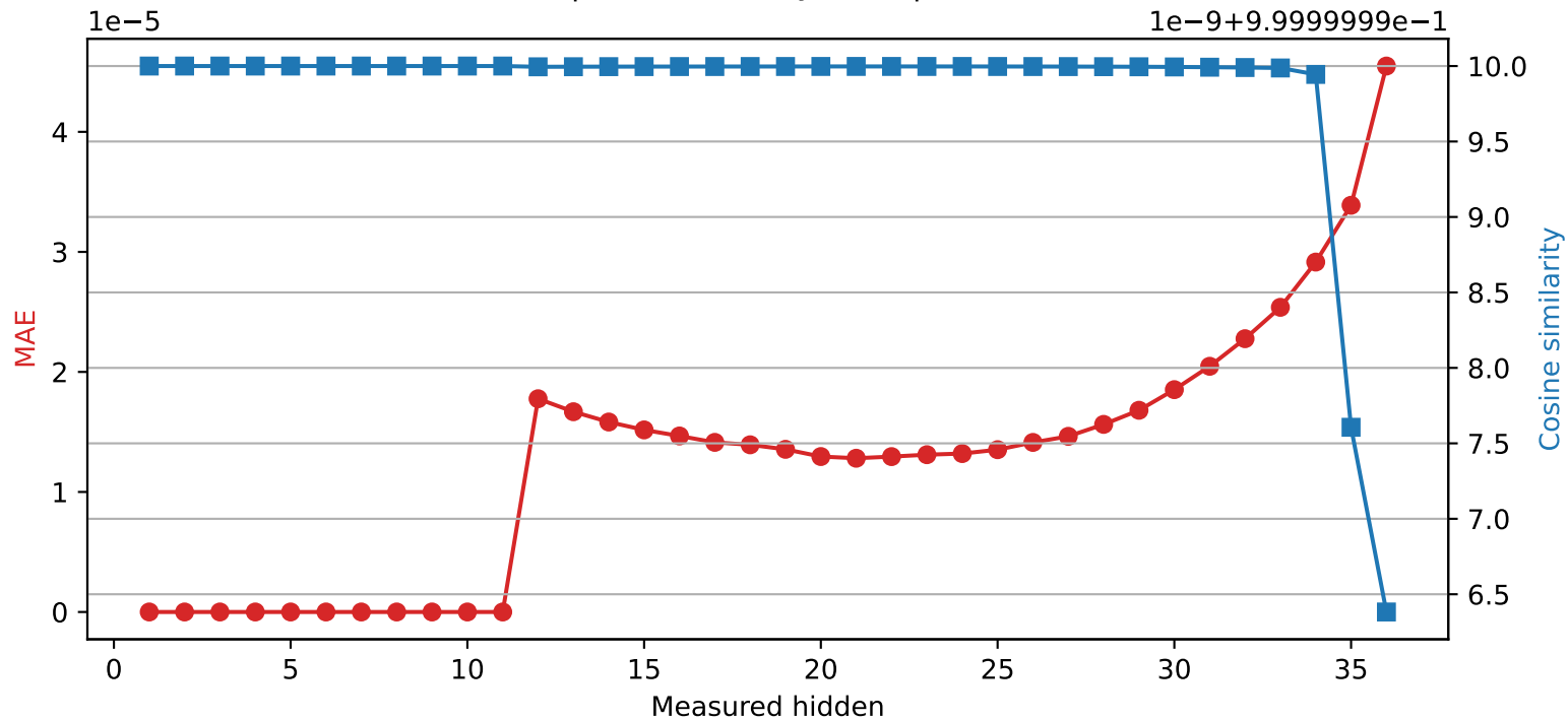
SmolLM3-3B | Quantized layer 11 | float64 → int16
