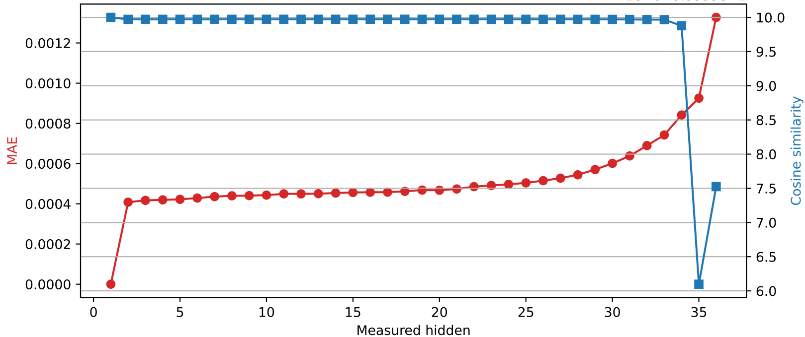
SmolLM3-3B | Quantized layer 1 | float64 → int16 1e-6 + 9.9999e-1
