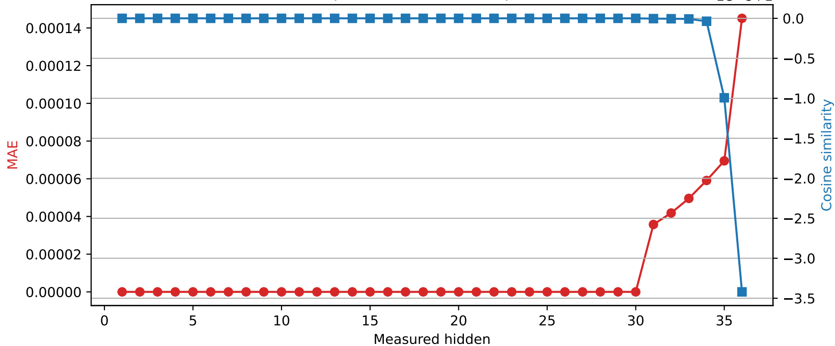
SmolLM3-3B | Quantized layer 30 | float64 → int16
