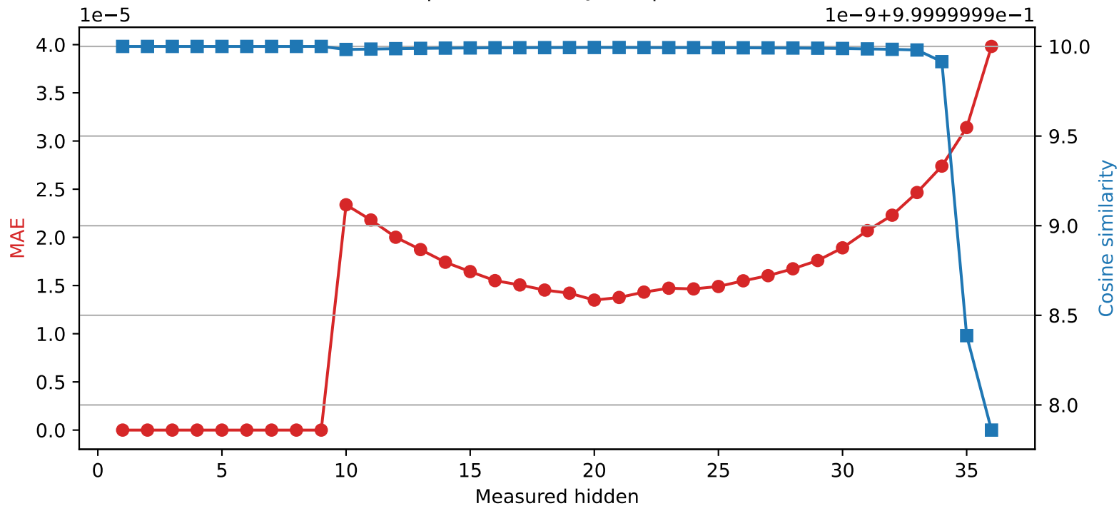
SmolLM3-3B | Quantized layer 9 | float64 → int16
