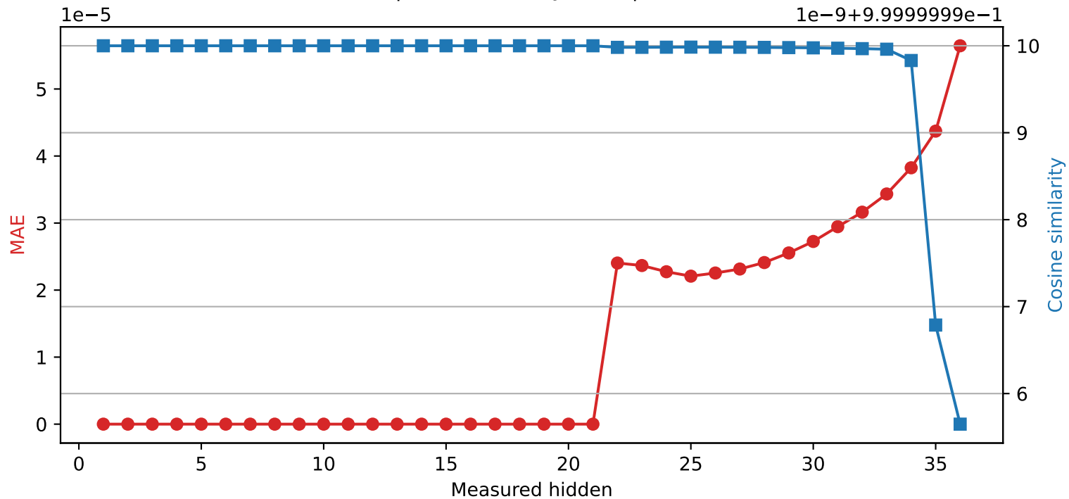
SmolLM3-3B | Quantized layer 21 | float64 → int16
