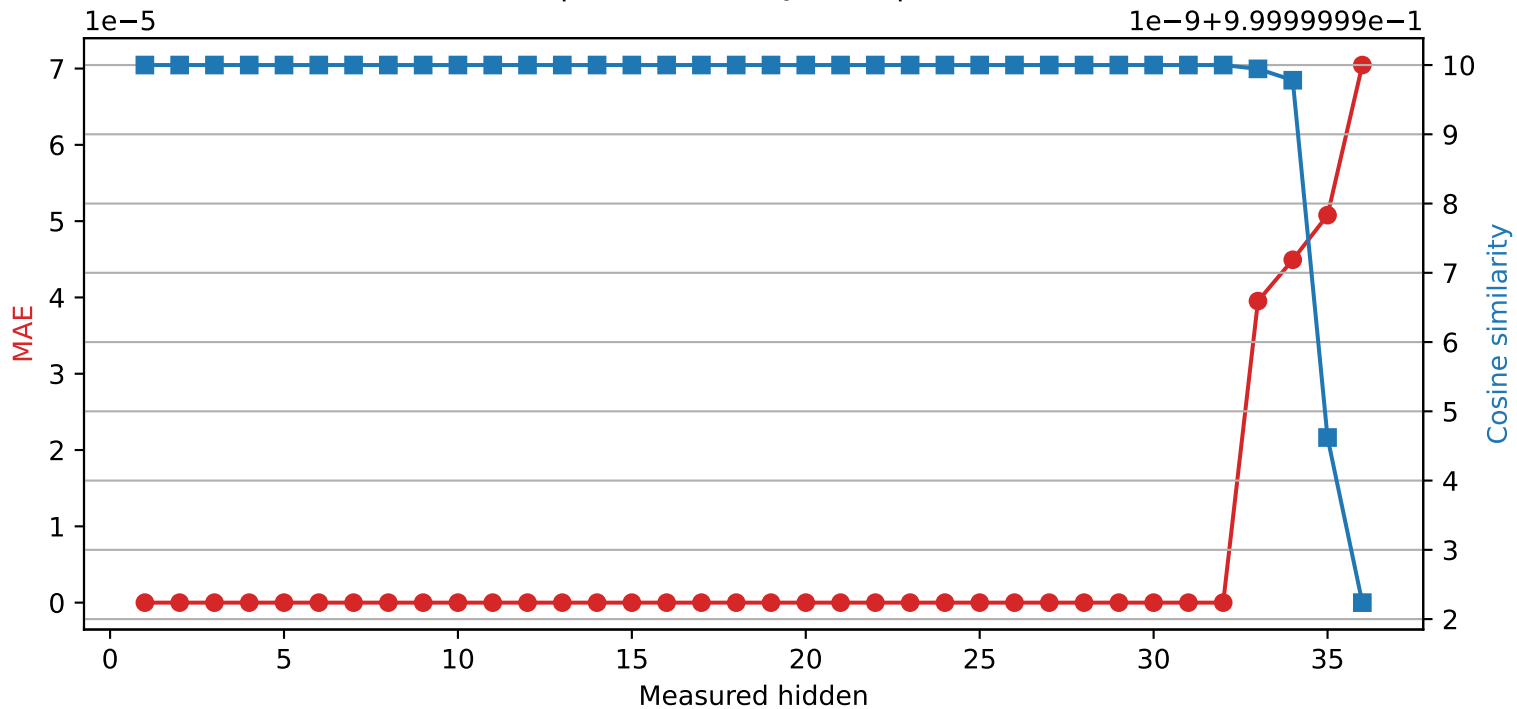
SmolLM3-3B | Quantized layer 32 | float64 → int16
