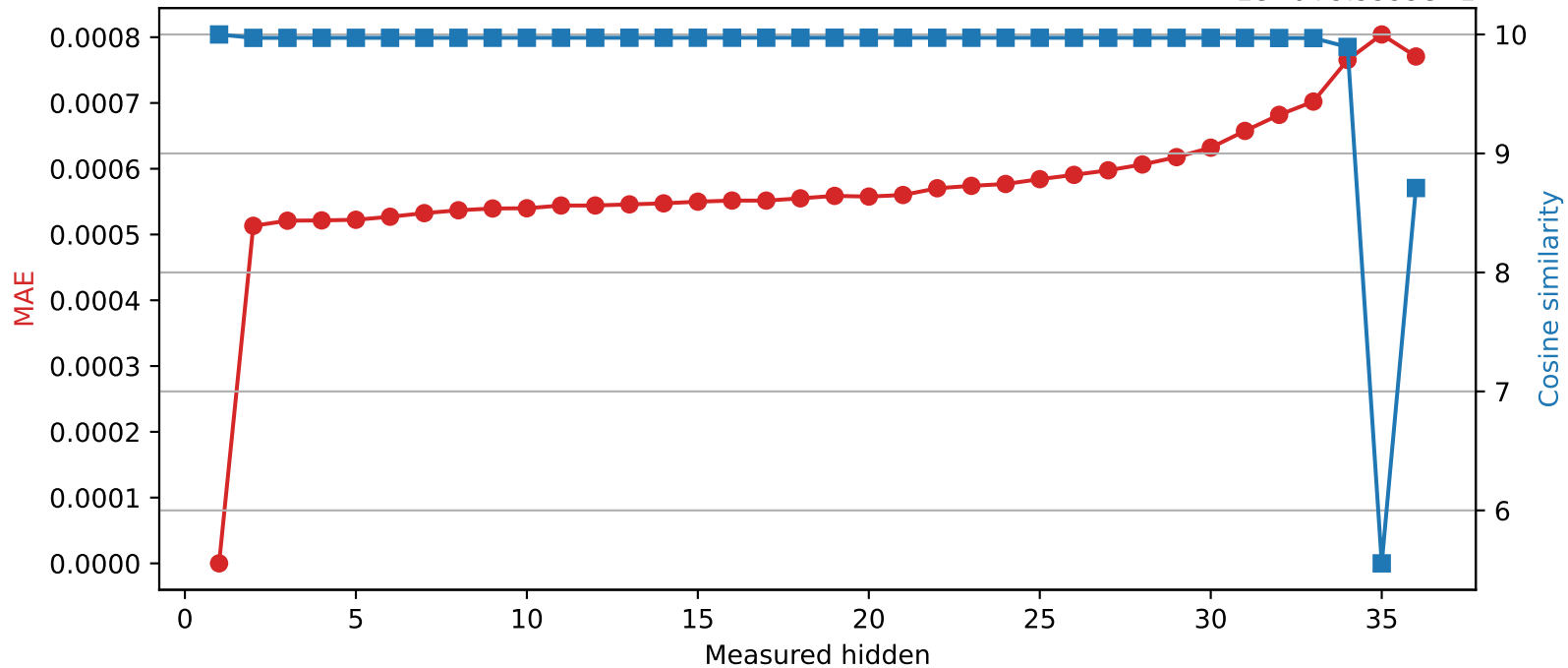
SmolLM3-3B | Quantized layer 1 | float64 → int16 1e-6+9.9999e-1
