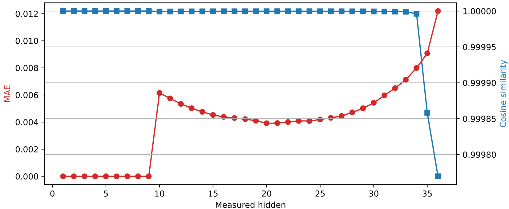
SmolLM3-3B | Quantized layer 9 | float16 \rightarrow int8
