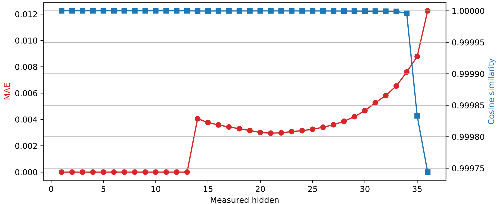
SmolLM3-3B | Quantized layer 13 | float16 → int8
