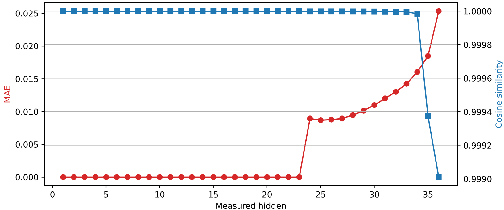
SmolLM3-3B | Quantized layer 23 | float16 \rightarrow int8
