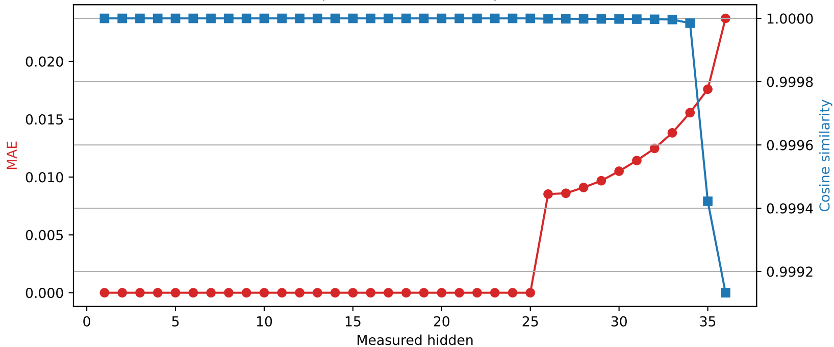
SmolLM3-3B | Quantized layer 25 | float16 \rightarrow int8
