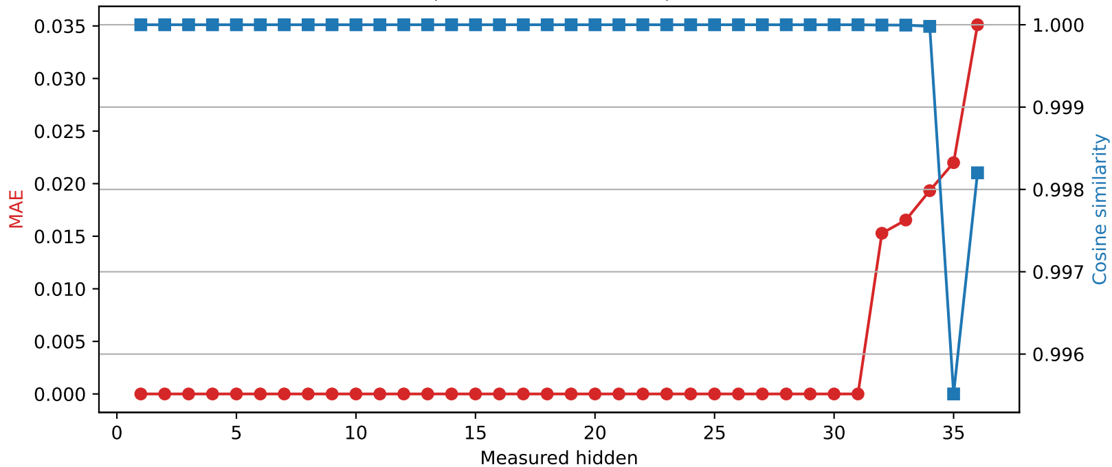
SmolLM3-3B | Quantized layer 31 | float16 → int8
