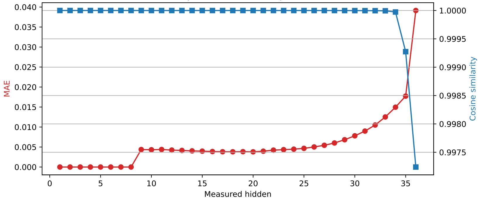
SmolLM3-3B | Quantized layer 8 | float16 \rightarrow int8
