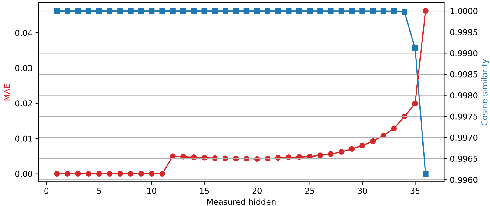
SmolLM3-3B | Quantized layer 11 | float16 → int8
