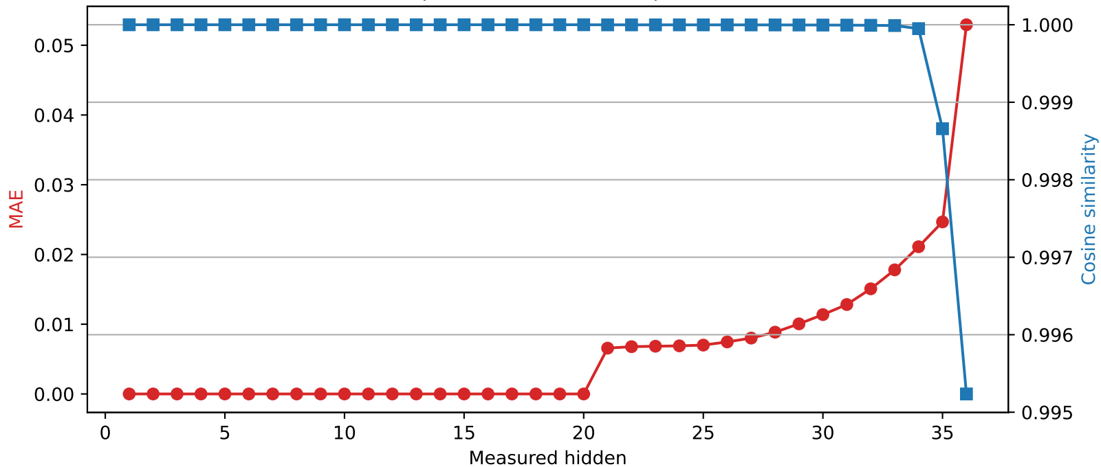
SmolLM3-3B | Quantized layer 20 | float16 → int8
