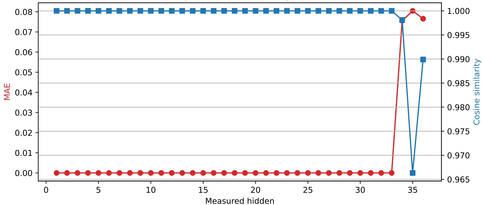
SmolLM3-3B | Quantized layer 33 | float16 → int8
