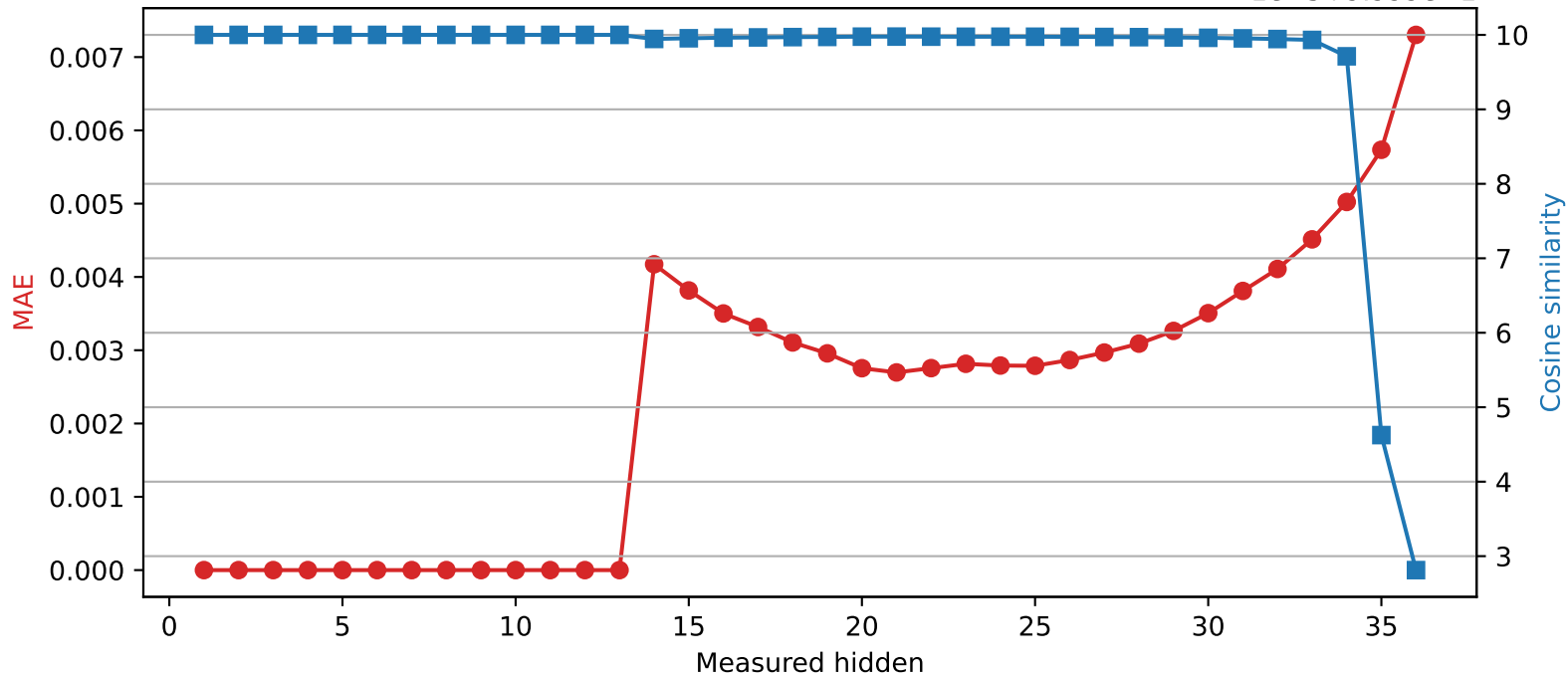
SmolLM3-3B | Quantized layer 13 | float16 → int8
