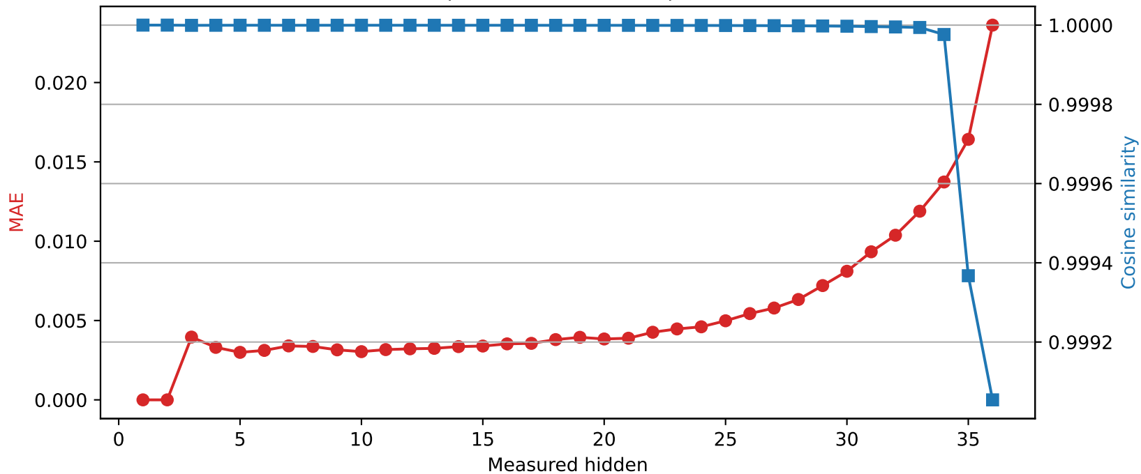
SmolLM3-3B | Quantized layer 2 | float16 \rightarrow int8
