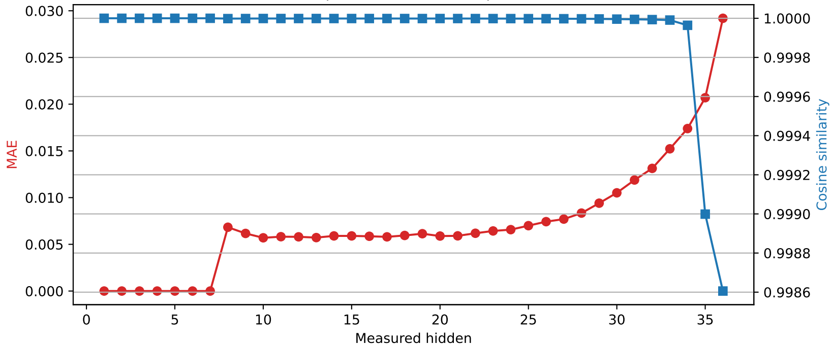
SmolLM3-3B | Quantized layer 7 | float16 → int8
