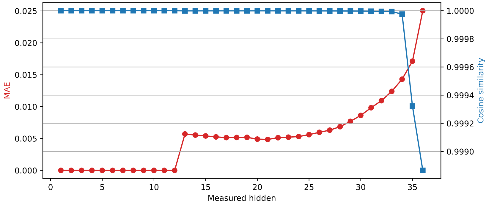
SmolLM3-3B | Quantized layer 12 | float16 \rightarrow int8
