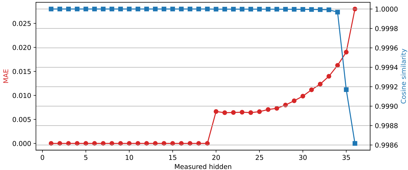
SmolLM3-3B | Quantized layer 19 | float16 \rightarrow int8
