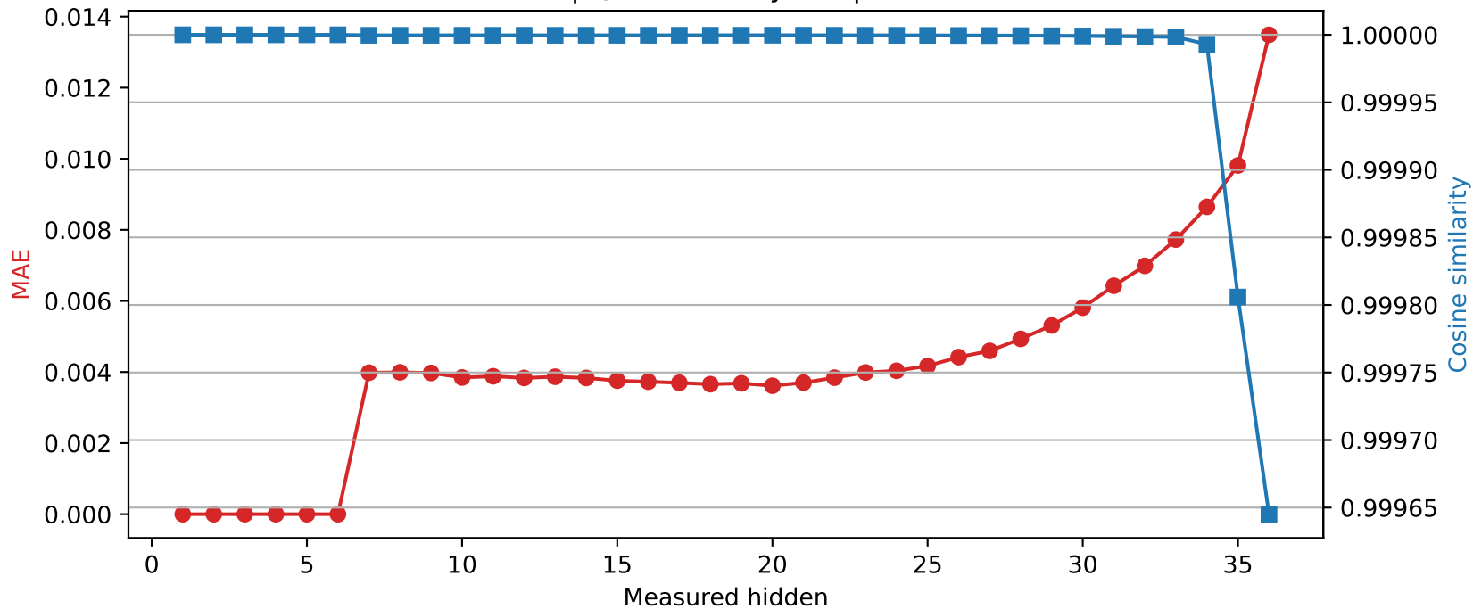
SmolLM3-3B | Quantized layer 6 | float16 → int8
