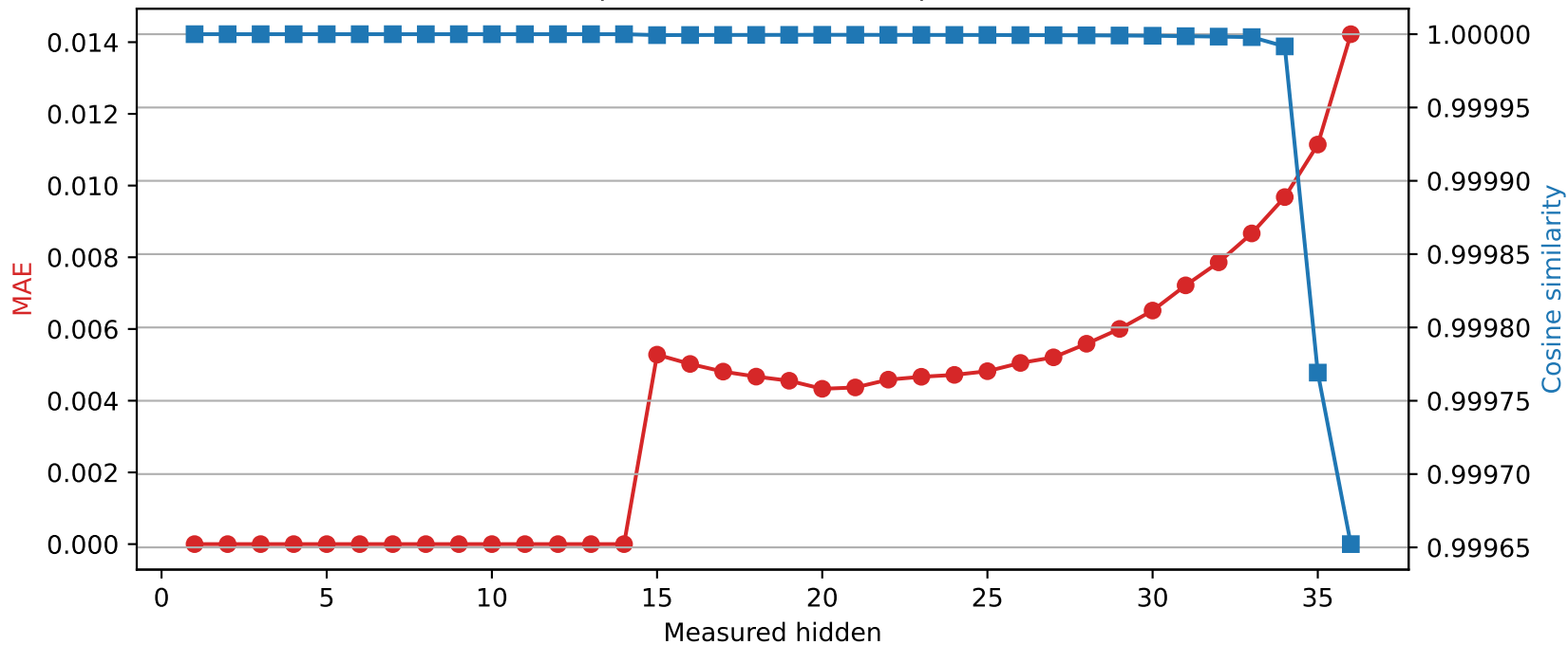
SmolLM3-3B | Quantized layer 14 | float16 → int8
