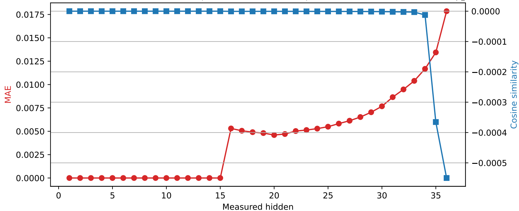
SmolLM3-3B | Quantized layer 15 | float16 → int8
