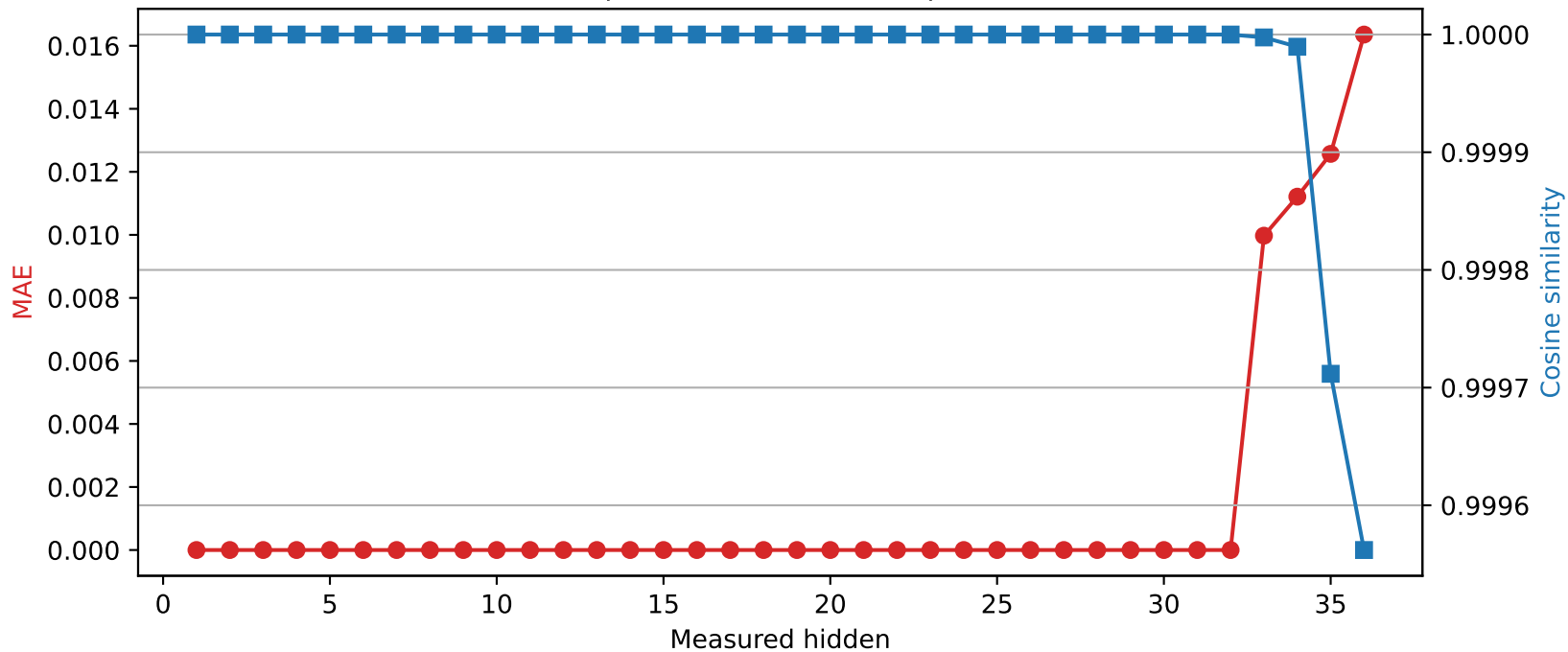
SmolLM3-3B | Quantized layer 32 | float16 \rightarrow int8
