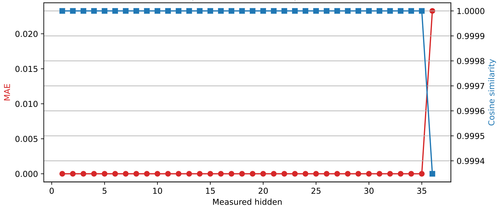
SmolLM3-3B | Quantized layer 35 | float16 → int8
