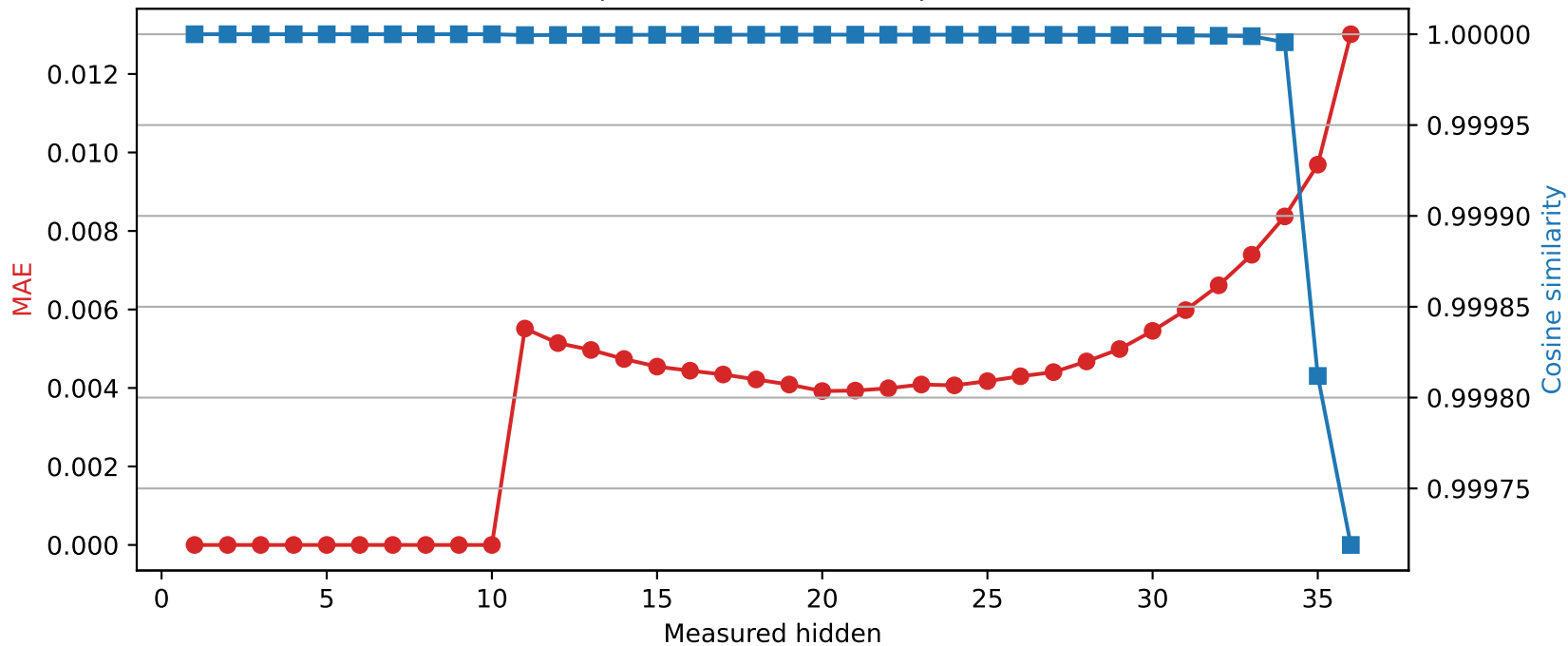
SmolLM3-3B | Quantized layer 10 | float32 → int8
