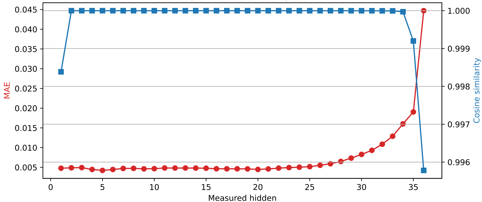
SmolLM3-3B | Quantized layer 0 | float32 \rightarrow int8
