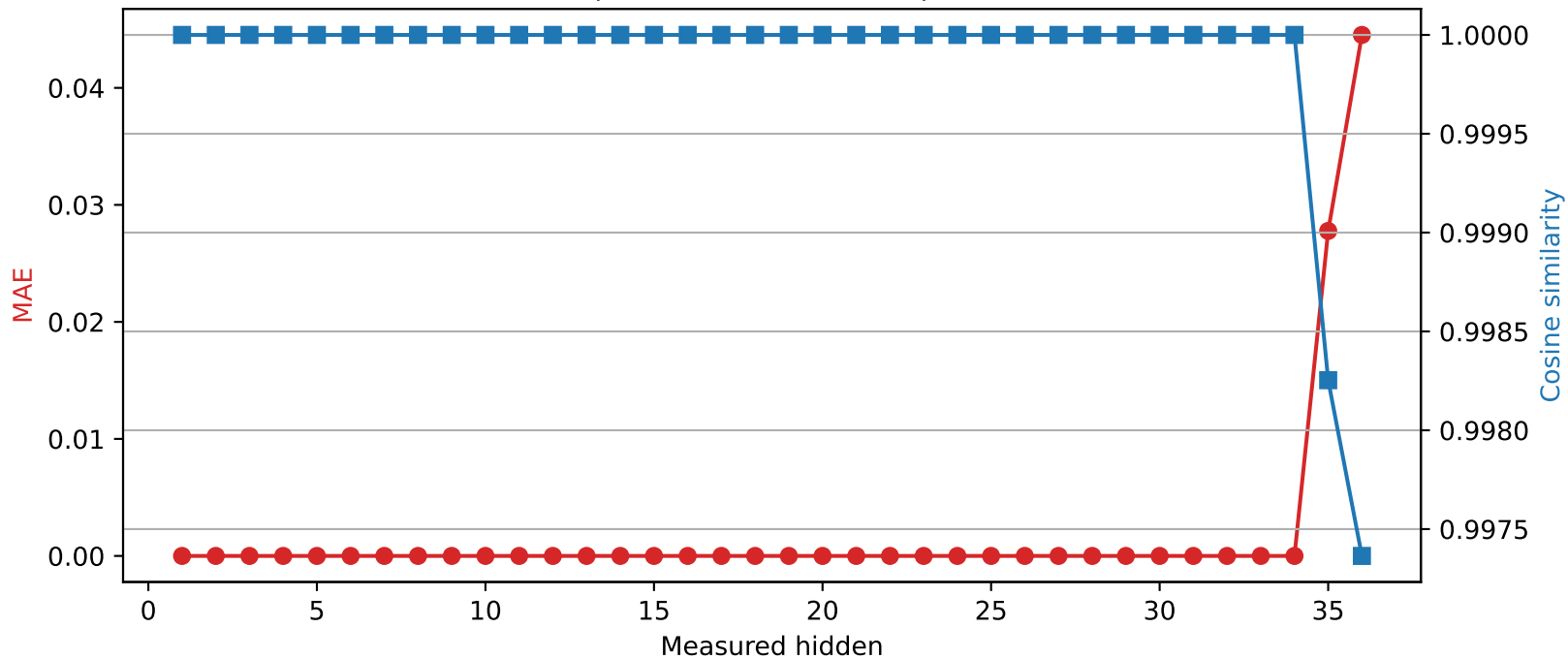
SmolLM3-3B | Quantized layer 34 | float32 → int8
