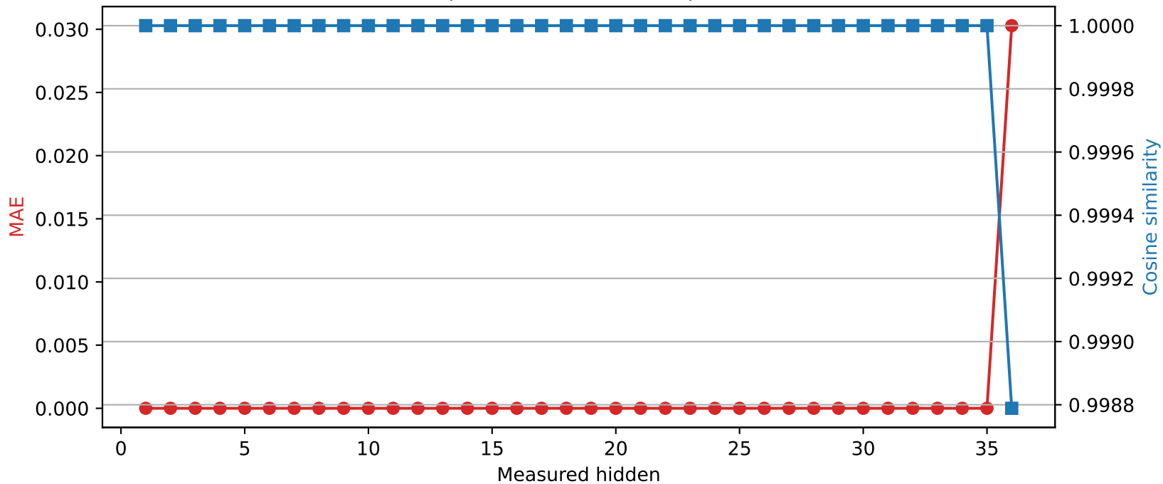
SmolLM3-3B | Quantized layer 35 | float32 → int8
