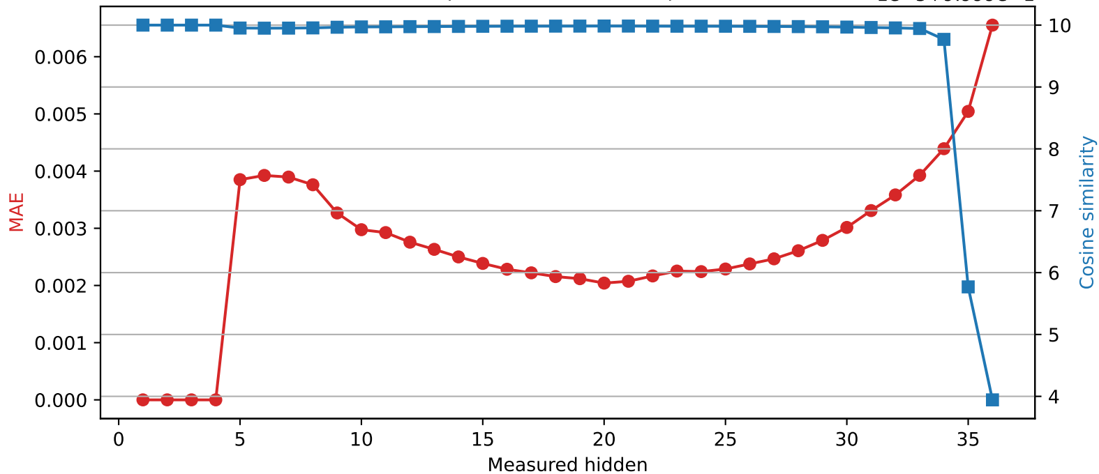
SmolLM3-3B | Quantized layer 4 | float32 → int8
