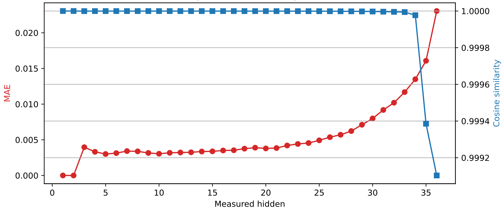
SmolLM3-3B | Quantized layer 2 | float32 \rightarrow int8
