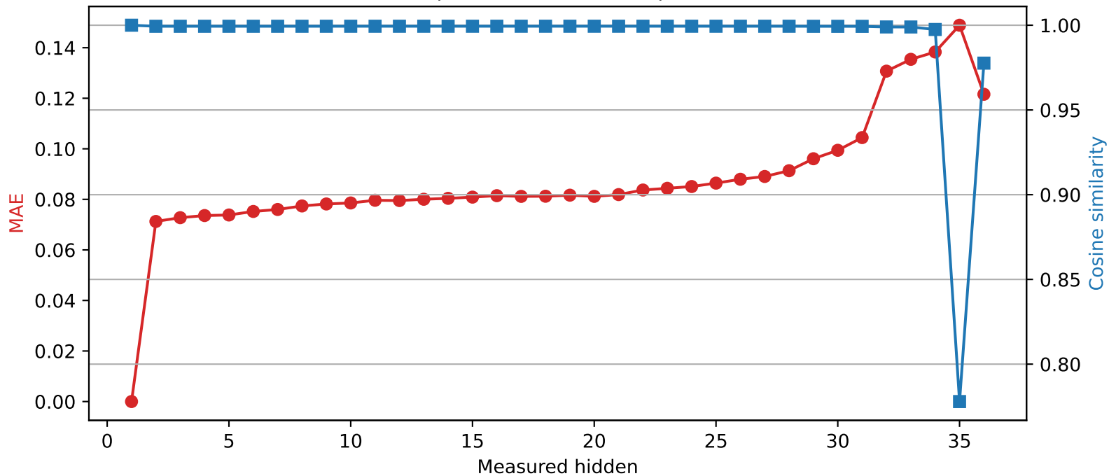
SmolLM3-3B | Quantized layer 1 | float32 → int8
