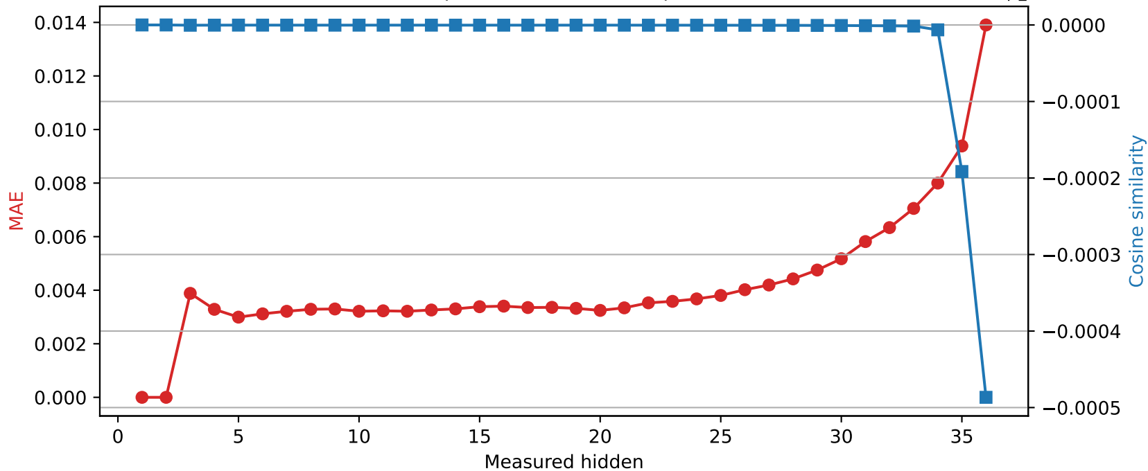
SmolLM3-3B | Quantized layer 2 | float32 \rightarrow int8
